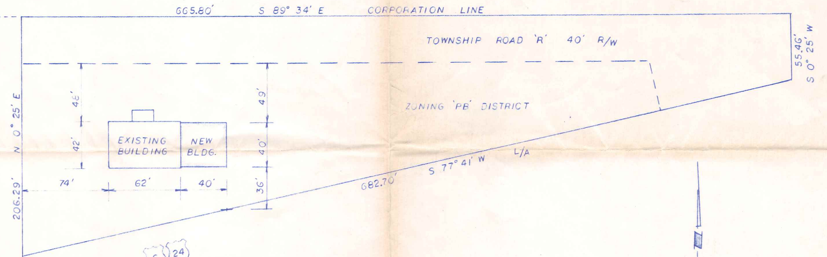
SITE PLAN 1" = 50'-0"
