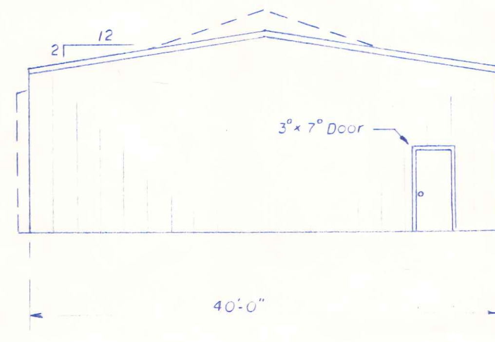
EAST ELEVATION 1/8" = 1'-0"
