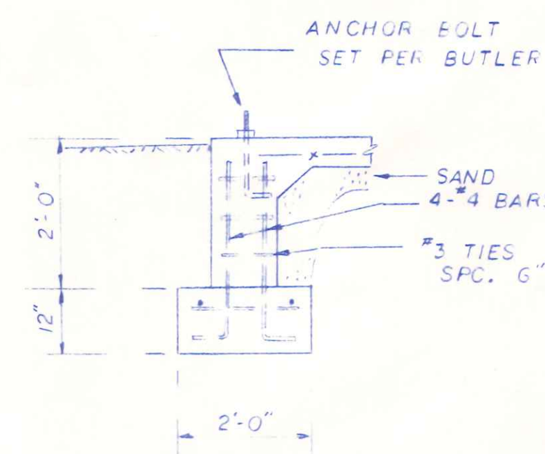
TYPICAL FOOTER
