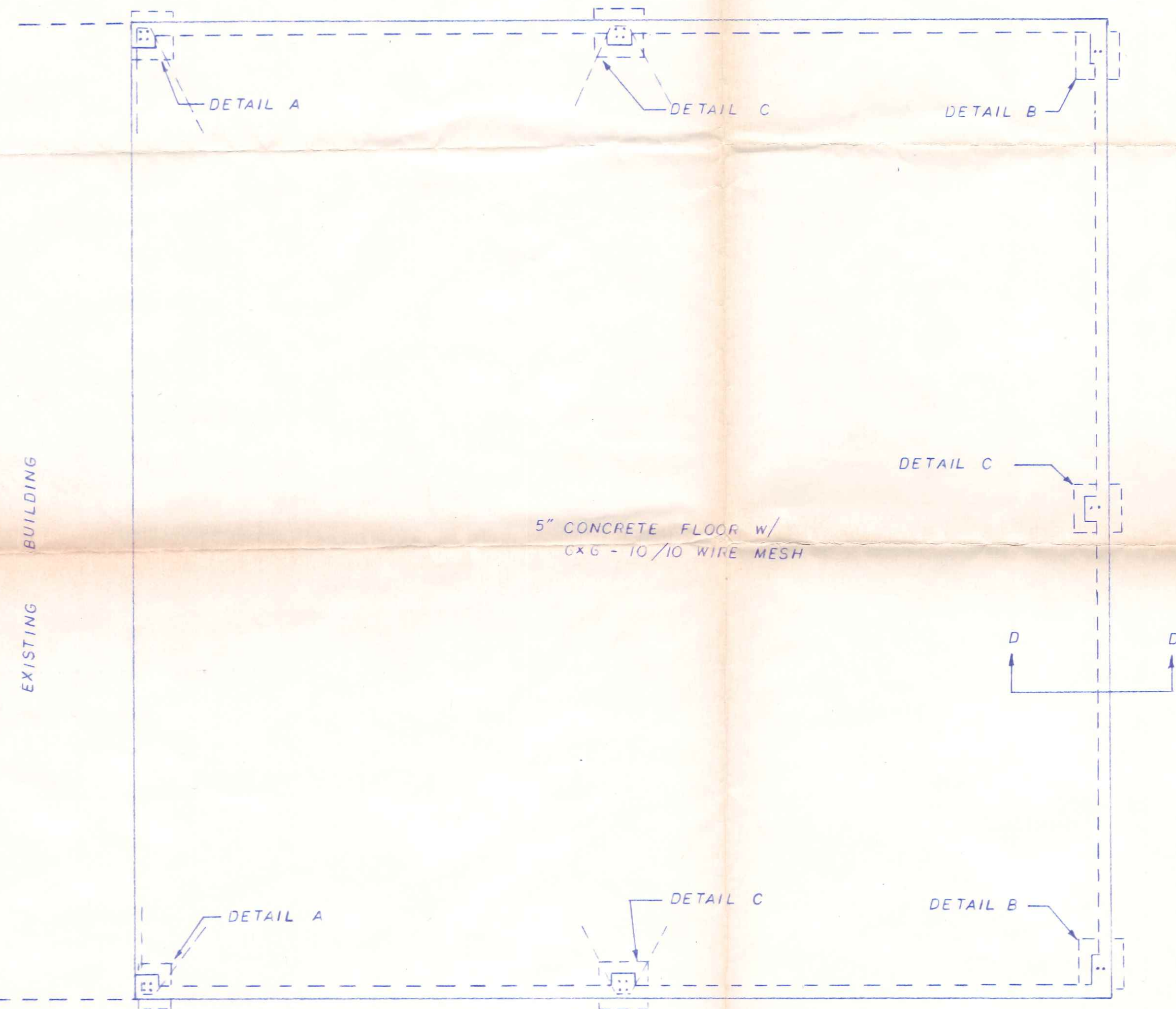
FOUNDATION PLAN 1/4" = 1'-0"
