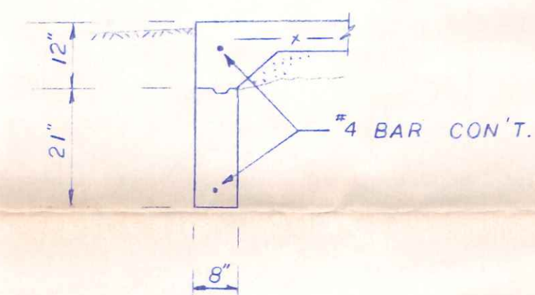
SECTION D
