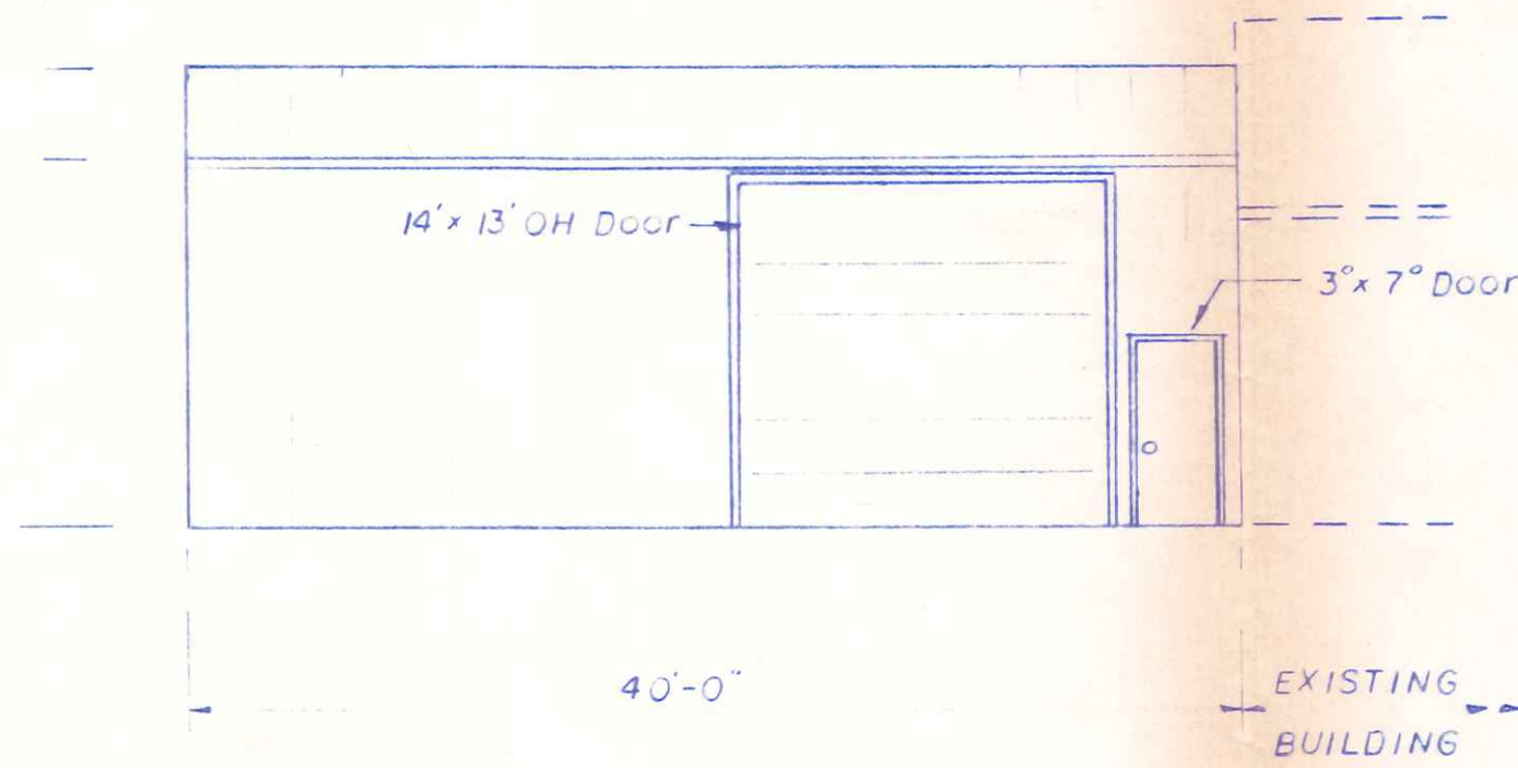
NORTH ELEVATION 1/8" = 1'-0"
