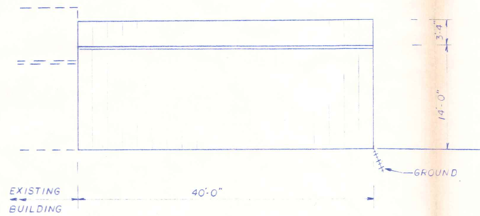
SOUTH ELEVATION 1/8" = 1'-0"
